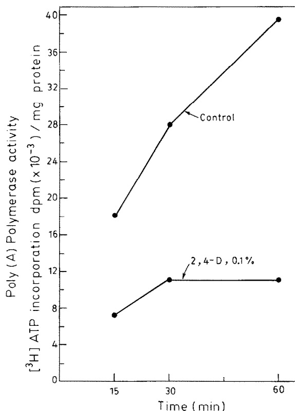
Fig. 1. [ ^3\text{H} ]ATP incorporation into the poly(A) product as a function of time in control and 2,4-D-treated pea epicotyl apices. Poly(A) polymerase activity was assayed in 'G-25 fraction'.
